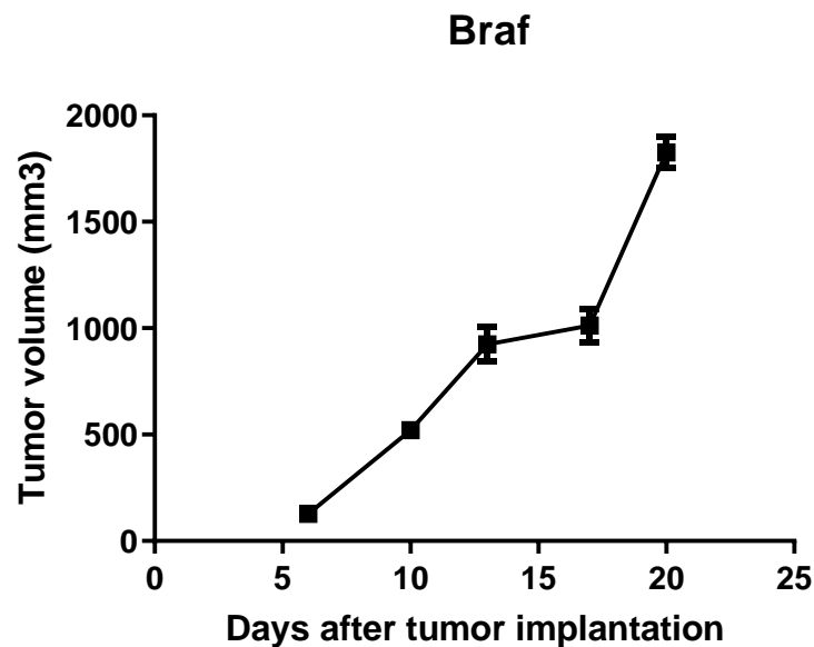
Figure 1: Tumour growth curve of the Braf cells as subcutaneous tumors Mean ± SEM (n=6; take rate 100%)
